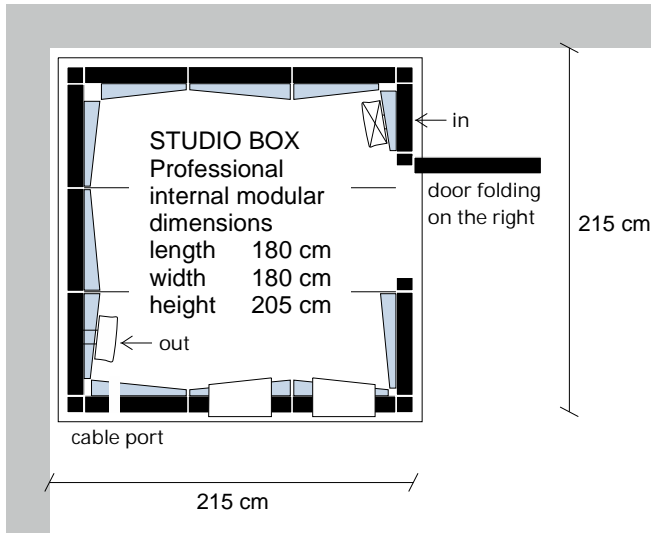
Planning Example - floor space required 215 cm x 215 cm
